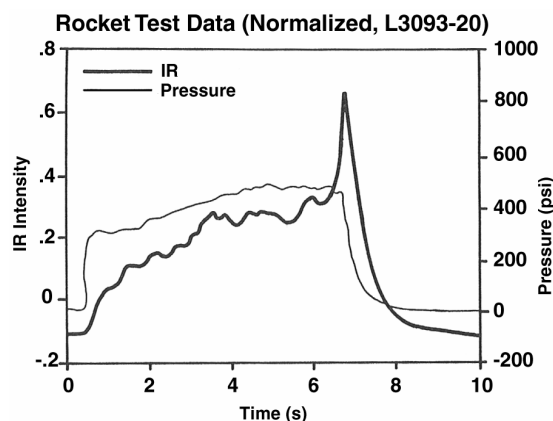
Figure 7. Carbon dioxide band infrared emission intensity and pressure data from a solid propellant taken using the fixed wavelength radiometer.
