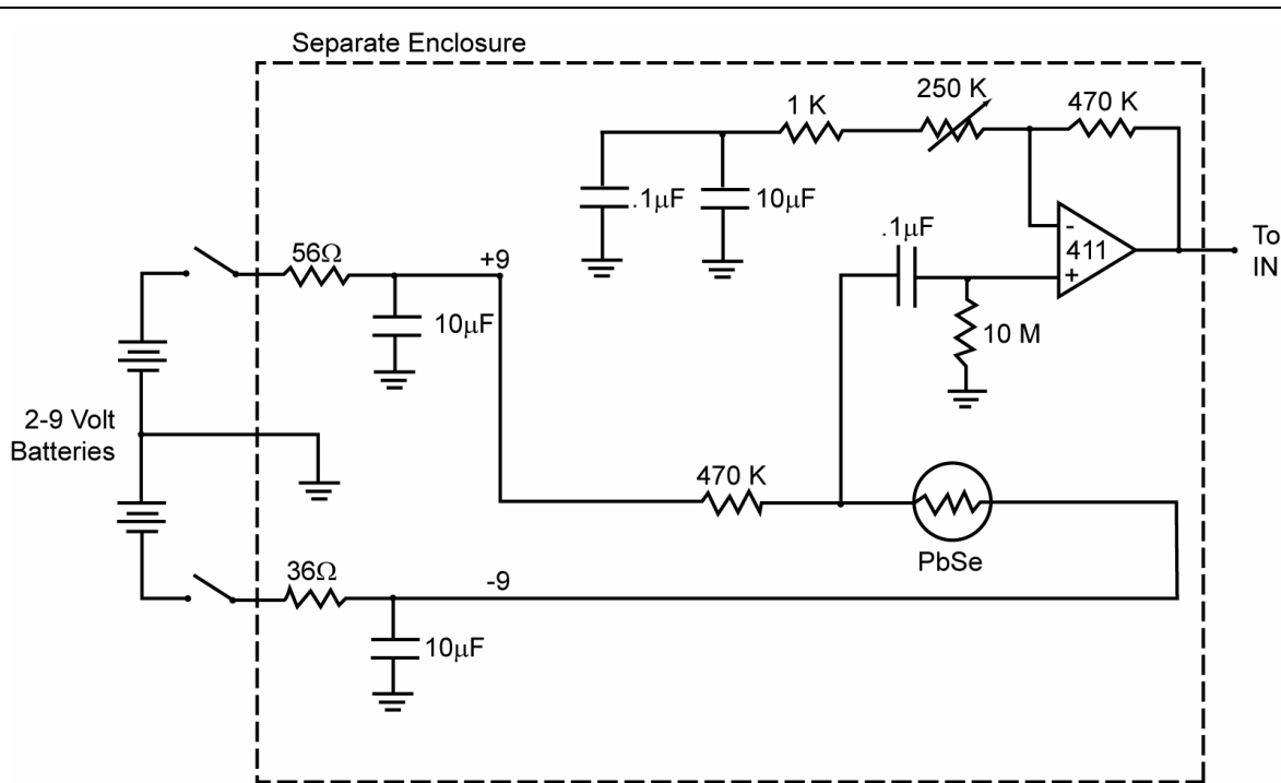
Figure 2. Detector and pre-amp circuitry.
