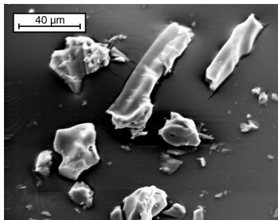
Figure 9. Particles with some rod-like characteristics (C) are produced by slow coacervation. Upper, 60 to 100 mesh (250 to 150 micron) particles at 100\times magnification; middle, a portion of one particle at 500\times magnification; lower, -400 mesh ( < 37 micron) particles at 500\times magnification.
