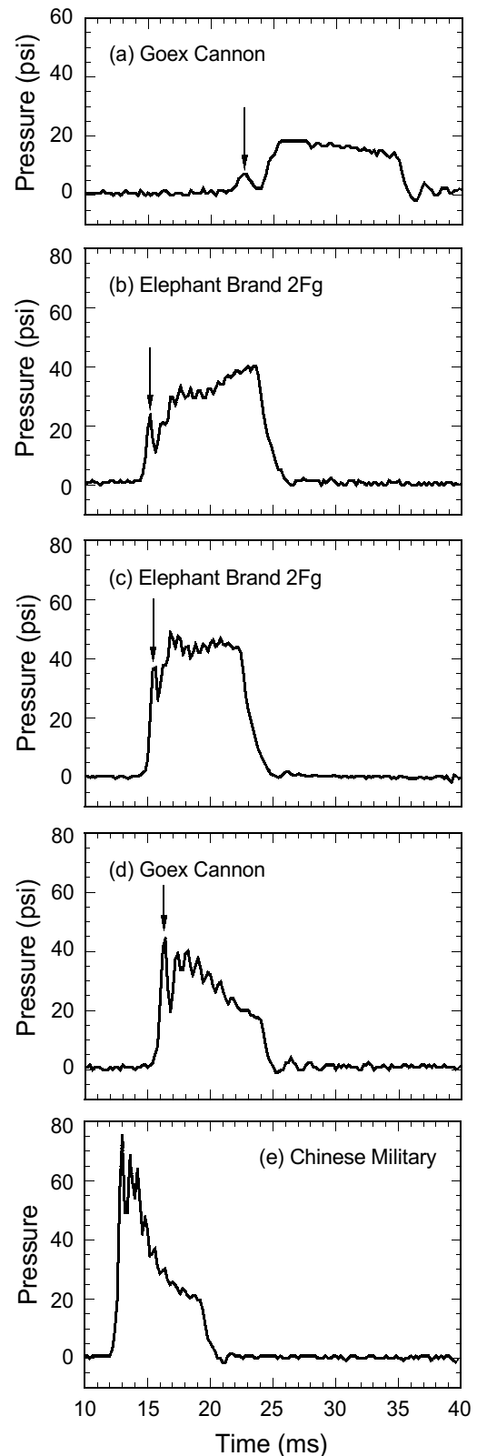
Figure 12. Examples of the precursor pressure peaks seen when firing slower burning powders.
