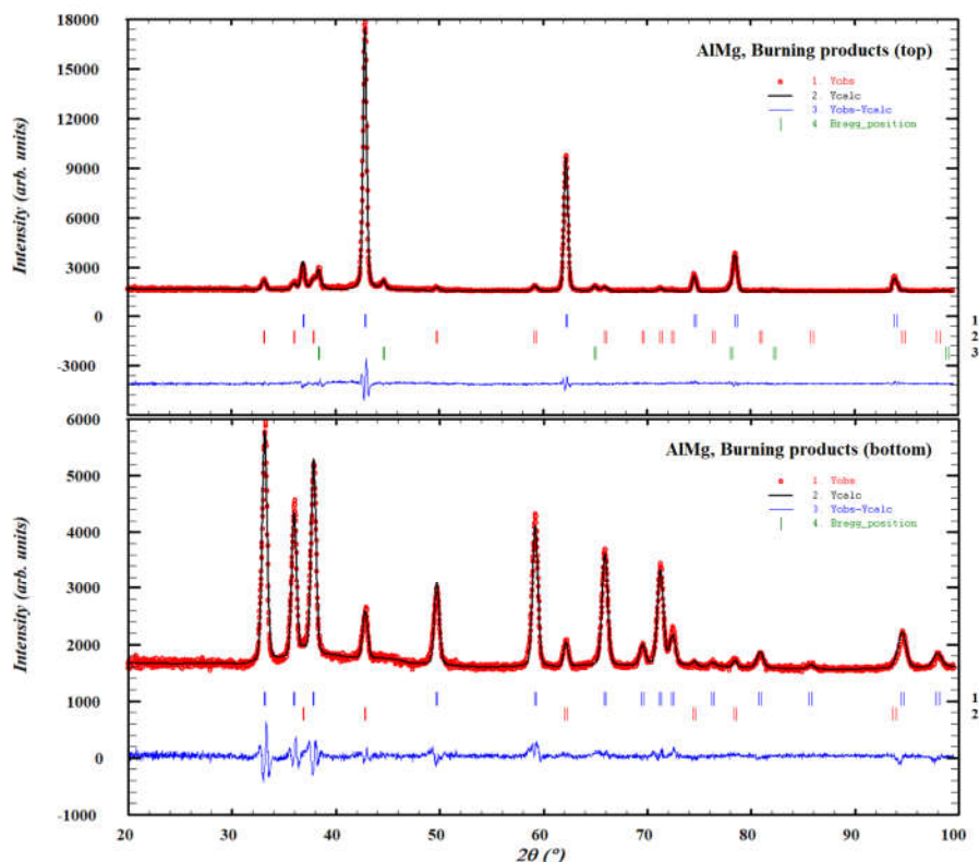
Figure 9. Refined powder X-ray diffraction patterns for the combustion products of magnalium at 850°C: (a) (1 - MgO, 2 - AlN, 3 - Al; R_p = 2.14\% , R_{wp} = 2.94\% ) and (b) (1 - AlN, 2 - MgO; R_p = 1.90\% , R_{wp} = 2.67\% ).
