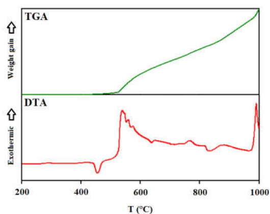
Figure 4. DTA/TGA curves for magnalium at a heating rate of 10^\circ\text{C}/\text{min} in air.
