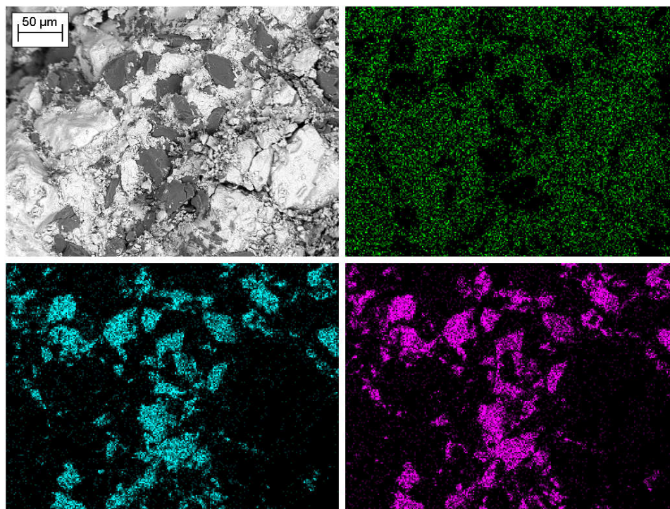
Figure 16. Microphotograph of the surface of the pressed \text{Ba}(\text{NO}_3)_2/\text{AlMg} pellet and the elemental distribution of barium (green), magnesium (blue) and aluminum (purple).
