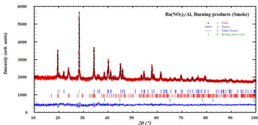
Figure 12. Refined powder X-ray diffraction patterns for the combustion products of \text{Ba}(\text{NO}_3)_2/\text{Al} (1 - \text{BaAl}_2\text{O}_4 , 2 - \text{BaCO}_3 , 3 - \text{Al} ; R_p = 1.44\% , R_{wp} = 1.88\% ).
