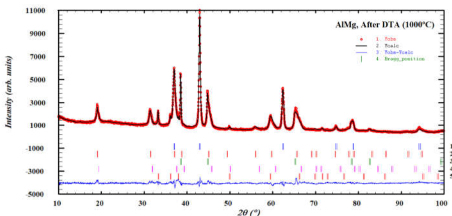
Figure 10. Refined powder X-ray diffraction patterns for the sintered products of magnalium after DTA/TGA up to 1000°C (1 - MgO, 2 - MgAl_2O_4 , 3 - Al, 4 - \gamma-Al_2O_3 , 5 - \alpha'-Al_2O_3 ; R_p = 4.43\% , R_{wp} = 5.78\% ).
