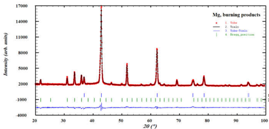
Figure 5. Refined powder X-ray diffraction patterns for the combustion magnesium powder at 850°C (1 - MgO, 2 - Mg 3 N 2 ; R p = 1.98%, R wp = 2.63%).
