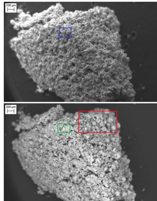
Figure 18. SEM images of the surface of a foam sample, using SE (top) and BSD (bottom) techniques.
